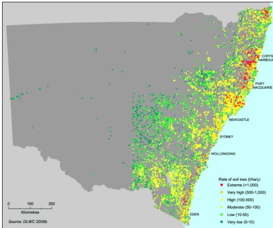
Figure 7.9. Inherent risk of sheet erosion by water in NSW soil profiles (Source: NSW EPA, 2000).
