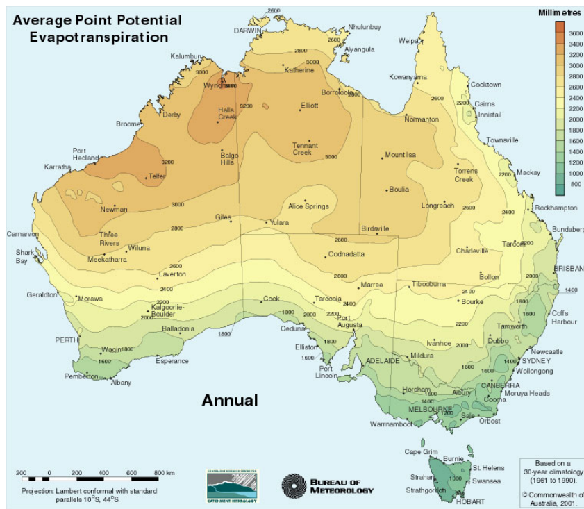
Figure 7.2 Average potential ET across Australia.
