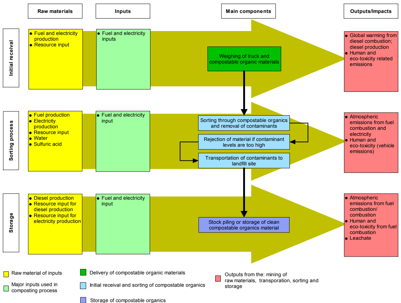
Figure 5.1 Sub-system model for compostable organic materials receive process in windrow composting system model.
